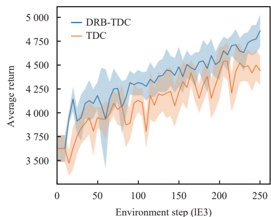
(b) Walker2d-medium-replay
