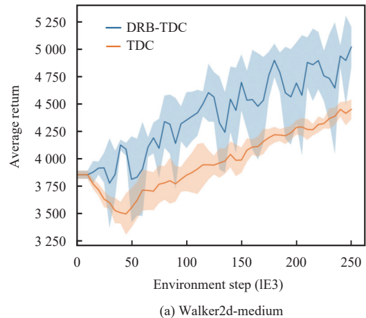
(a) Walker2d-medium
